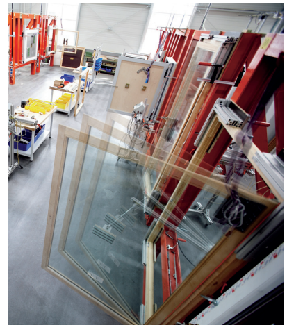
20,000 tilt cycles and up to 30,000 turn cycles: the most important NT components are tested beyond the current standards and guidelines.
