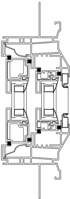
Top View
